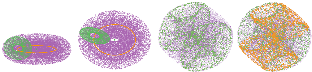
Figure 18: Several views of torii: (two at left) 4D ring torus, and (two at right) 6D flat torus. In each case, a subset has been highlighted which illustrate the low-dimensional donut shapes. Adapted from Schloerke et al., 2016, Figures 10 and 13.
