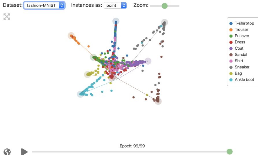
Figure 15: A grand tour run on the output of a deep neural network model for classification. The axes correspond to the probabilities that the model of an image belonging to a certain class. Adapted from Li et al., 2020.
