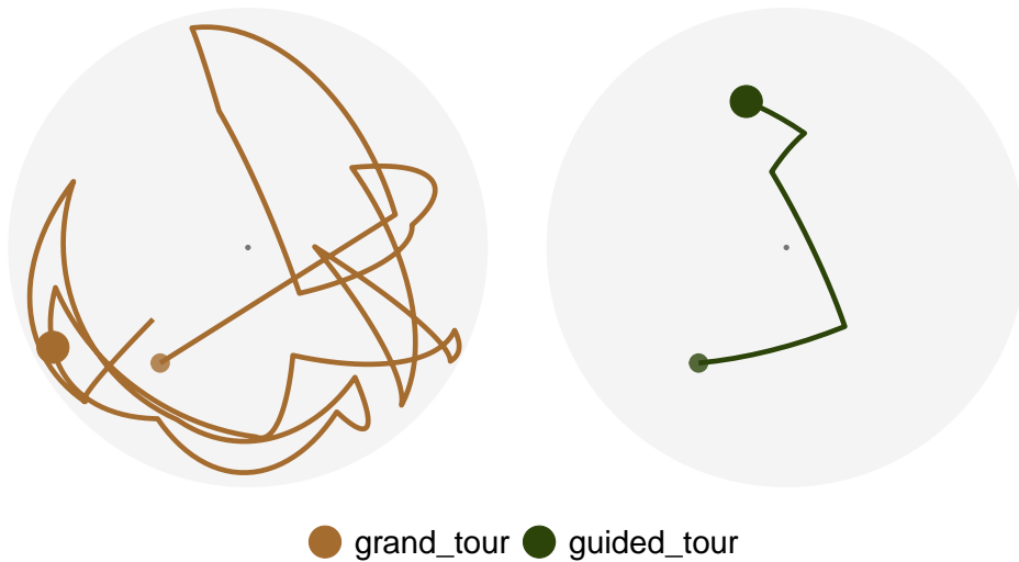
Figure 6: A comparison of guided and grand tour path in the PCA reduced 2D space. The start point of tour paths is smaller and lighter than the end point. Guided tour optimises the index value iteratively and finishes the search quickly while grand tour wanders in the parameter space to look at possible interesting projections.
