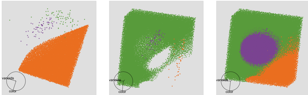
Figure 14: A grand tour run on the prediction boundaries of a radial support vector machine. (Left) The prediction region for points classified as orange produces a slice of a cube. (Middle) The prediction region for points classified as green produces another slice of the cube. (Right) The complete prediction region shows the points classified as purple are embedded within the green slice. Adapted from Wickham et al., 2015, Figure 6.
